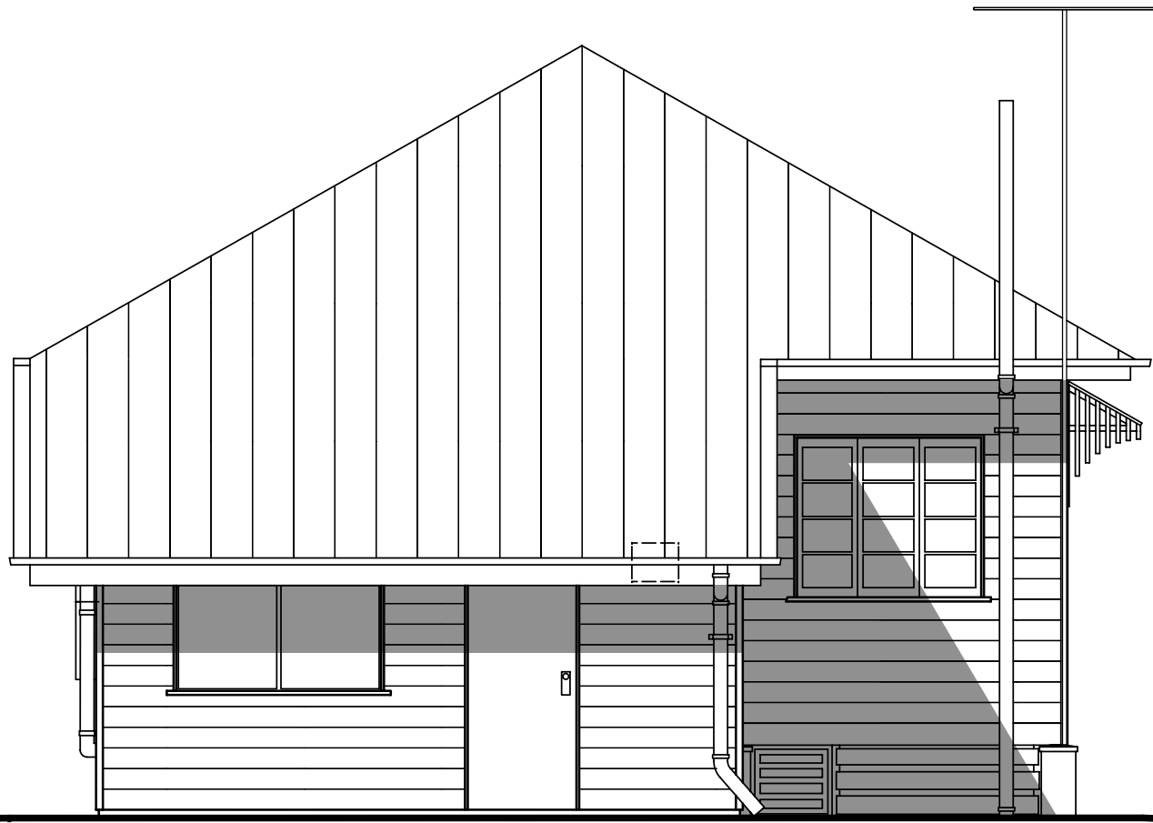
Elevation West - M 1:50
